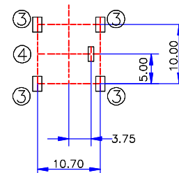
PCB MOUNTING HOLE
